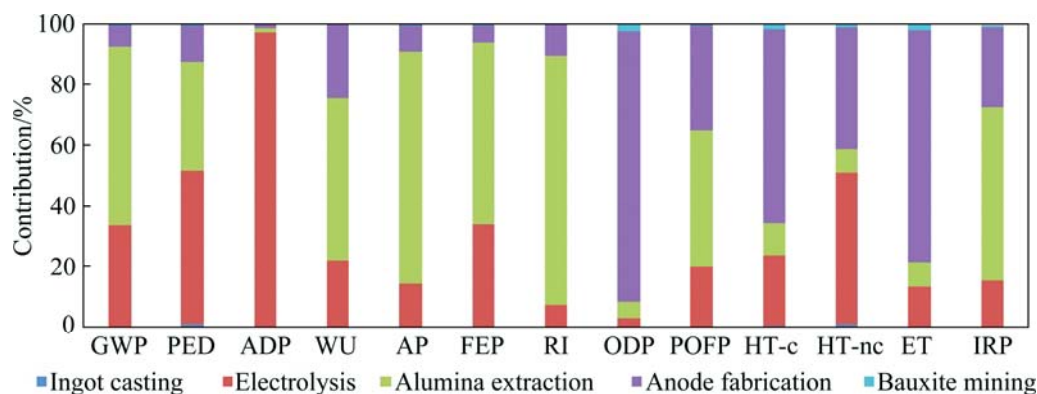
Fig. 3 Contributions to environmental impact categories of LCA-AI-HP
